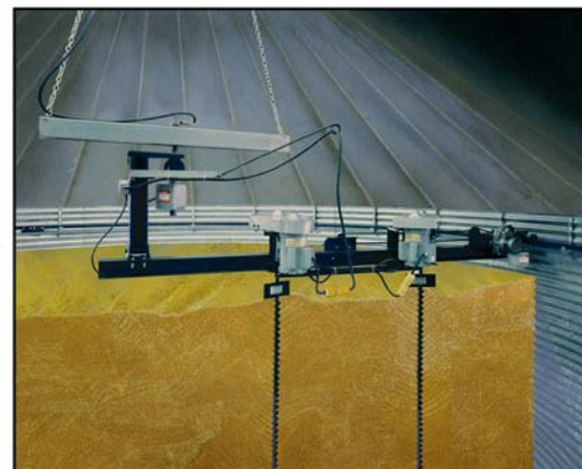
In-bin drying systems for farm or small capacity commercial applications.
