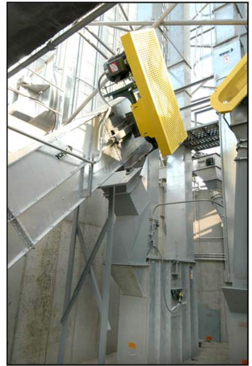
Bucket Elevators up to 1,500 MT/HR capacity.
